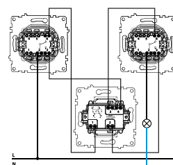
Wiring diagram for three-way control using one intermediate switch 1E3145130x and two two-way switches 1E3140130x.
