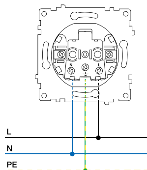
Electrical connection of the socket 1E1010130x-E, 1E1020130x-E, 1E1050130x-E Front view
