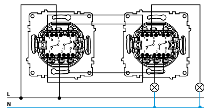
Schematic diagram of controlling two lights from 2 locations using 2-gang two-way switches (two switches 1E3160130x-E are needed)
